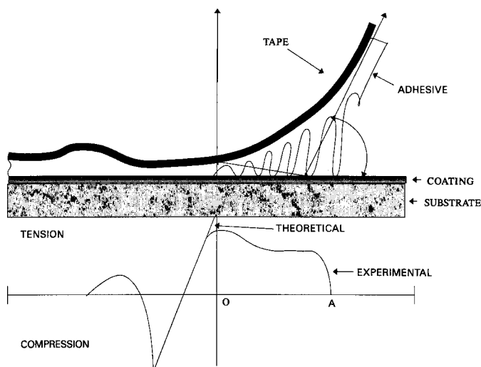
FIG. X1.1 Peel Profile (6)
